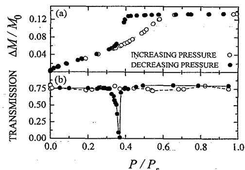
FIG. 2. (a) Hexane sorption isotherm and (b) transmission of light through Vycor. The lines are guides for the eye.
