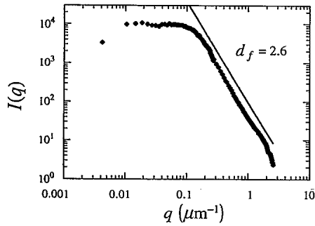
FIG. 3. Dependence of scattered light intensity on wave vector, illustrating the fractal correlations of the empty pores. The fractal dimension is d_f \approx 2.6 , as indicated by the slope of the solid line.
