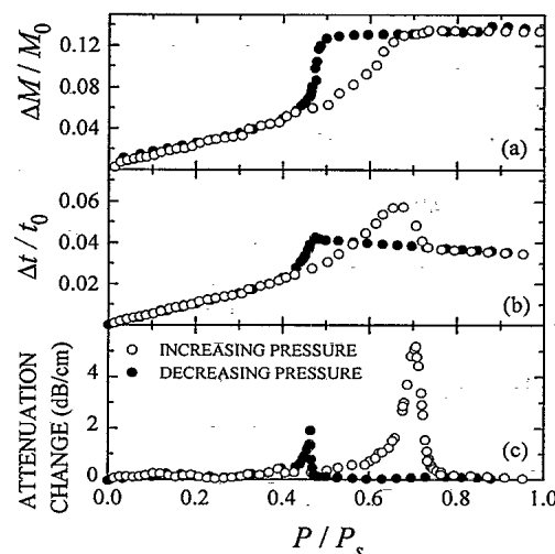
FIG. 1. (a) Hexane sorption isotherm, (b) relative change in the ultrasonic transit time, and (c) change in the ultrasonic attenuation for Vycor.
